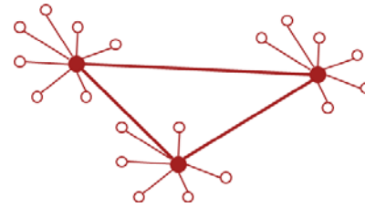
Network Management
